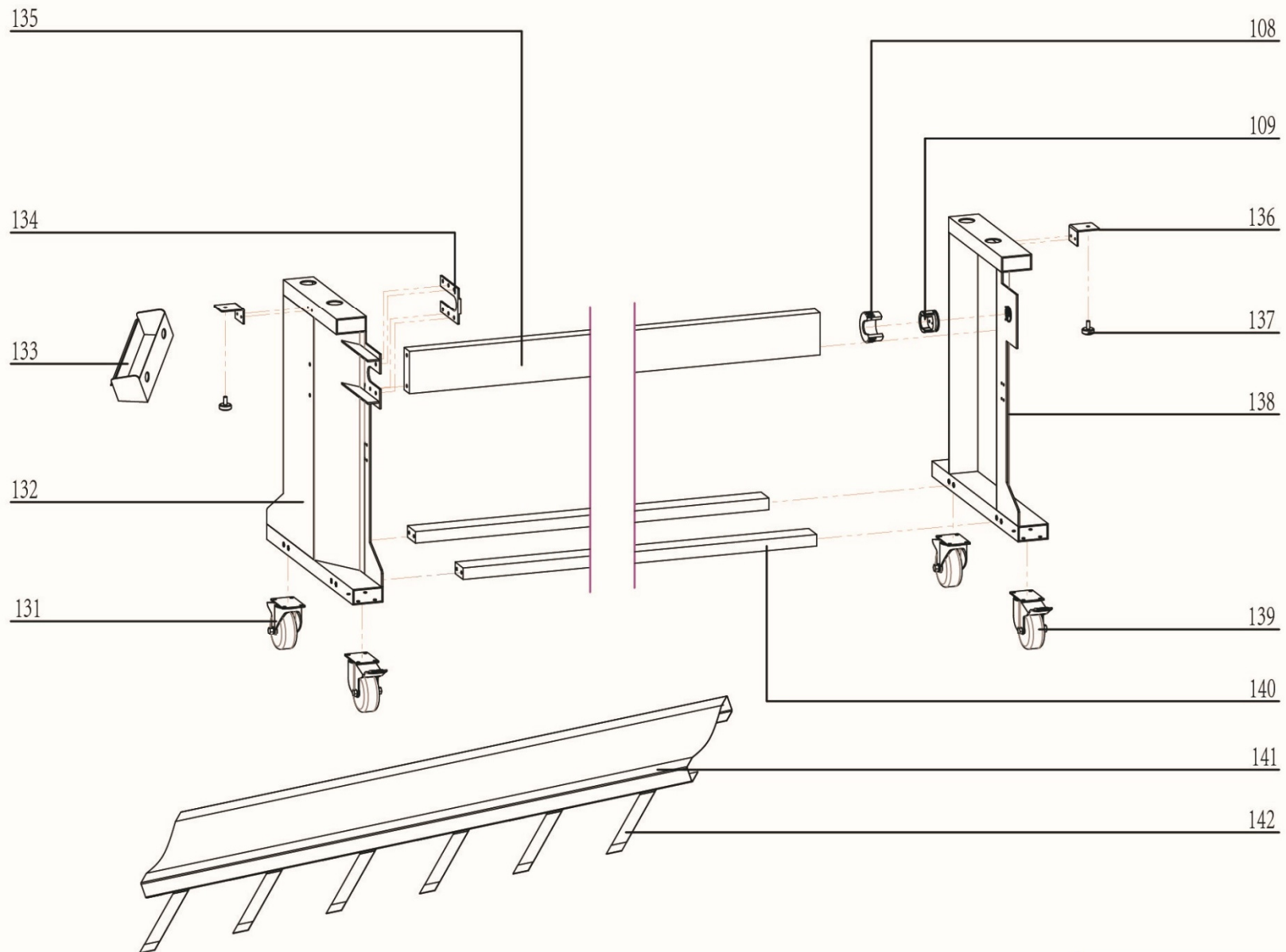
View11 - Stand and Blanket Assemblies
