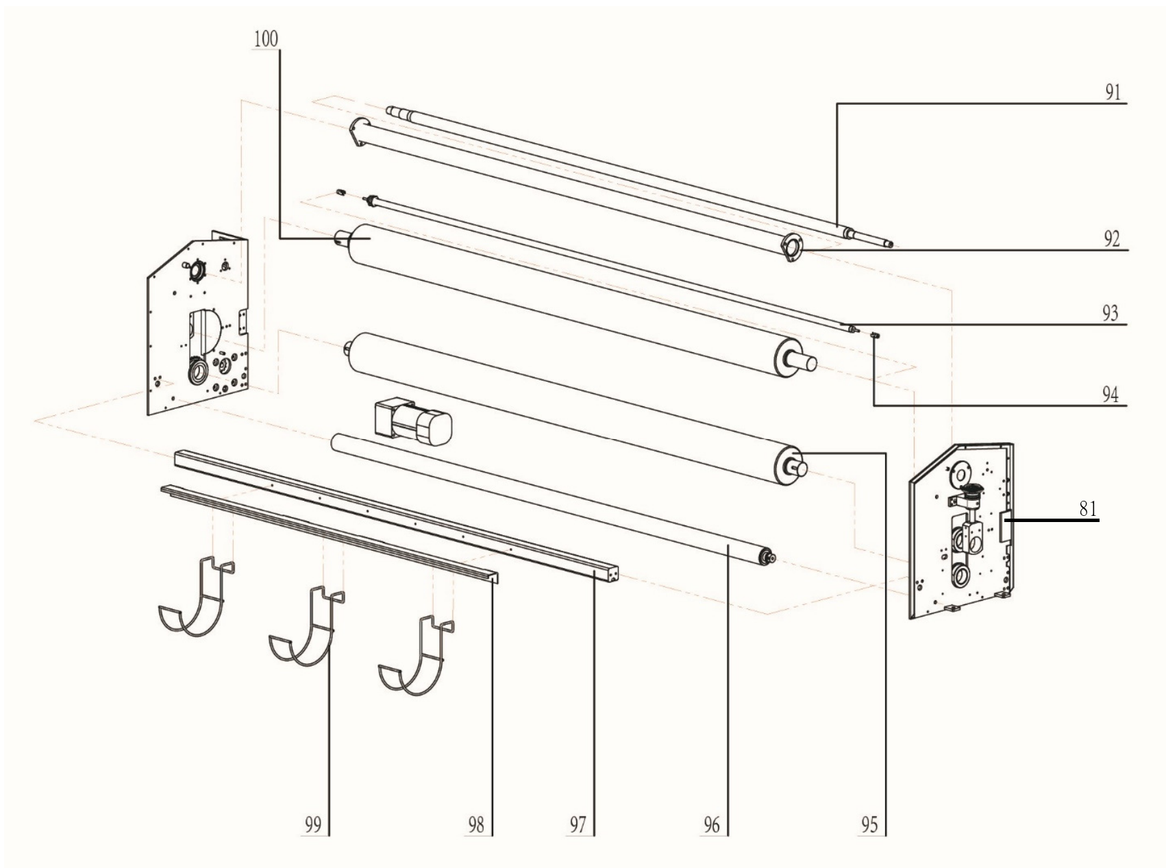
View 9 - Rollers, Cross Members, Media Baskets
